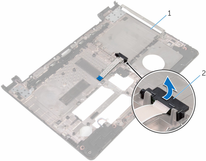
1 optical-drive interposer
